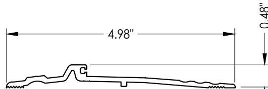
40 THRESHOLD
