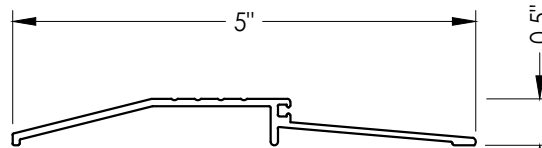
41 THRESHOLD
