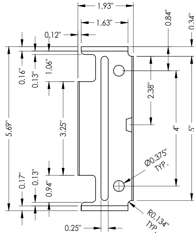
31 UNIVERSAL WALL ANCHOR
