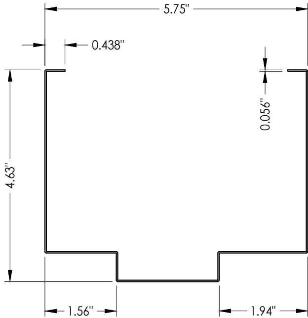
26 FRAME
